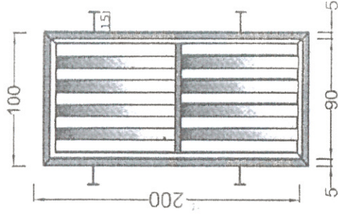
BACK VIEW OF DOOR
