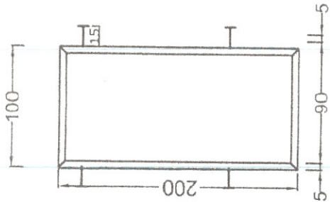
OUTSIDE FRAME OF DOOR
