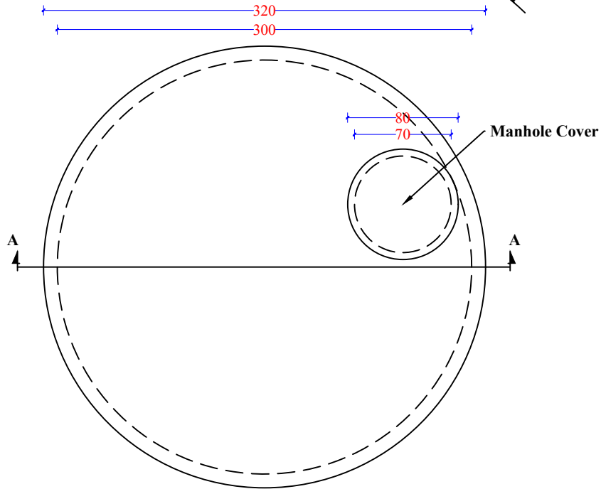
Plan of Large Diameter Dug Well
