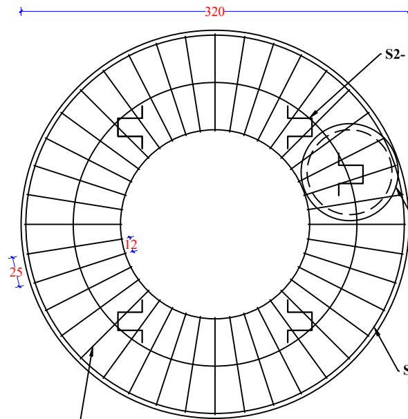
Plan of Top Reinforcement
