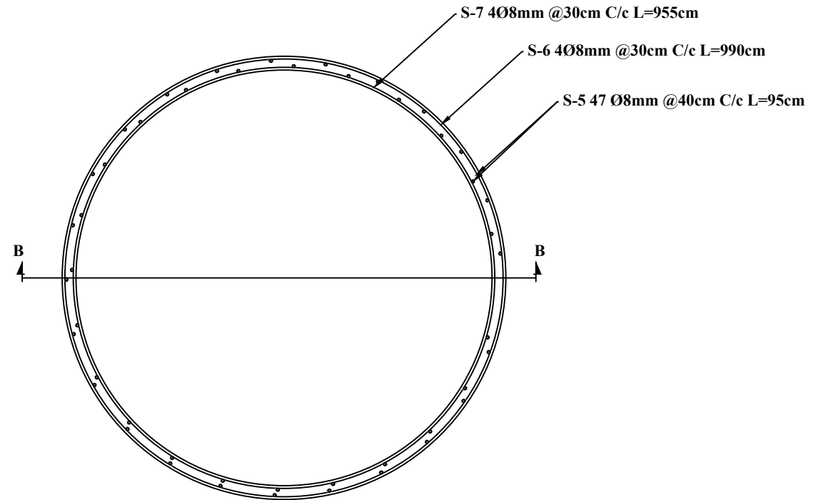
Plan of RCC Rings No= 16
