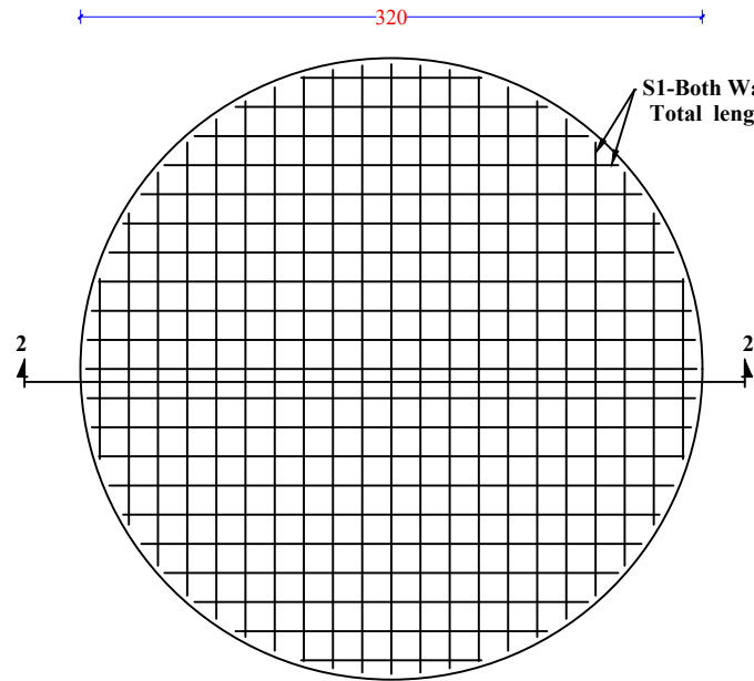
Plan of Bottom Reinforcement
