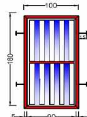
SQUARE IRON TUBE (ONE EDGED PROFEEL) FOR INNER FRAM (40mmX40mm) 18 Gauge THICK
