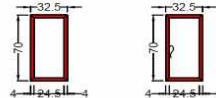
SQUARE IRON TUBE (ONE EDGED PROFEEL) (40mmX40mm) 18 Gauge THICK
