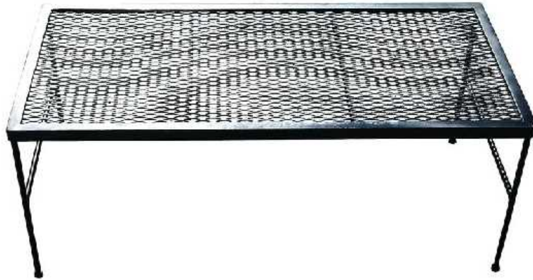
Figure 8: Burger colder lace/Table with mesh top (70*180 cm and 100 cm height and 4*4 cm hollow iron bar of 2 mm thickness)
