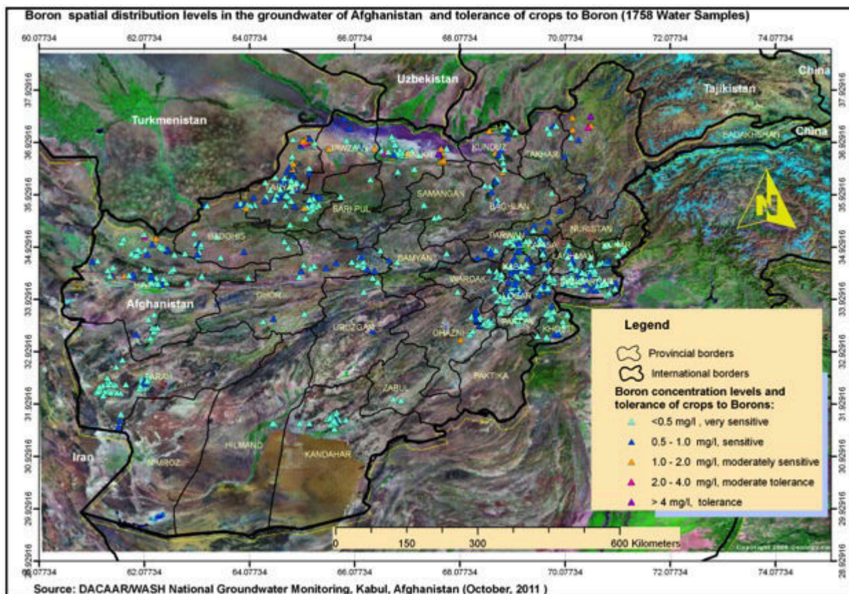
Figure 89 Boron distribution
