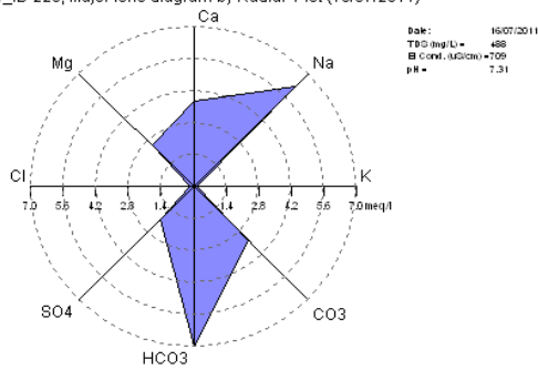
GMW_ID 220, Major ions diagram by Radial Plot (16/07/2011)
