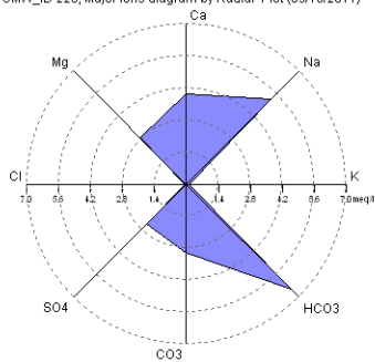
GMW_ID 220, Major ions diagram by Radial Plot (09/10/2011)
