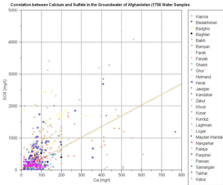
Figure 54 SO4 versus Ca
