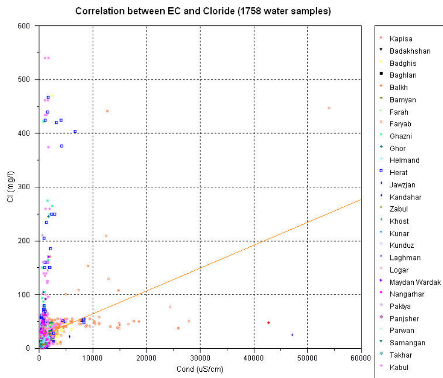
Figure 40 EC versus CI
