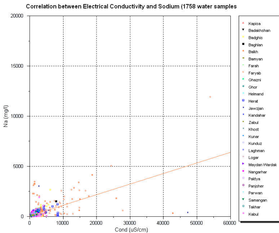
Figure 36 EC versus Na
