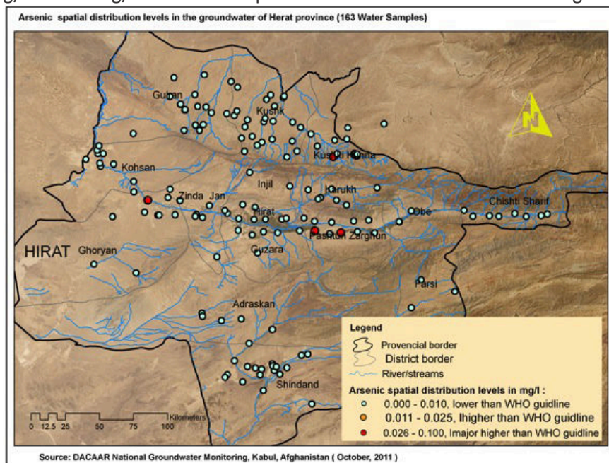
Figure 77 Arsenic contamination in Herat Province
