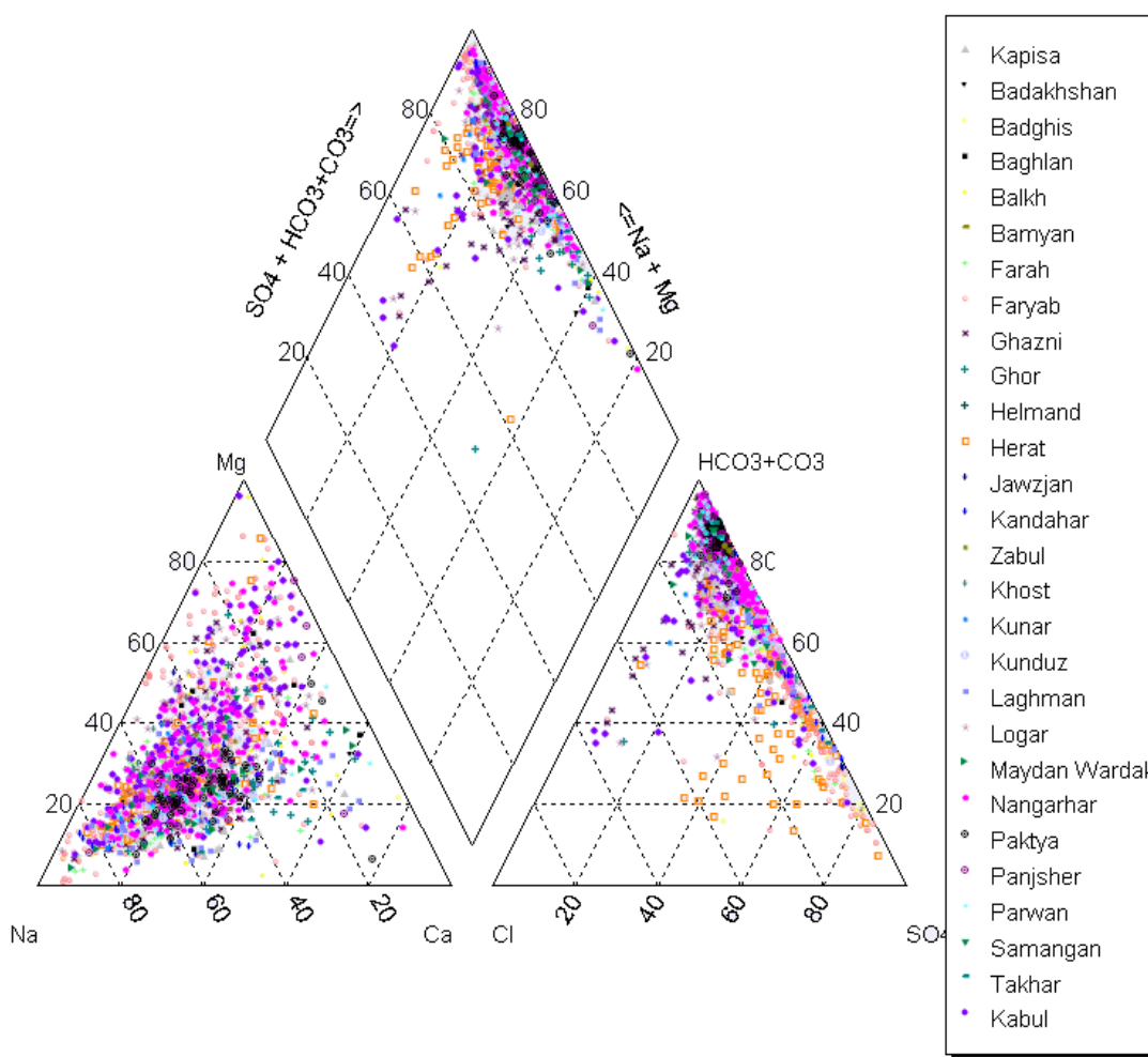
Figure 42 Piper diagram groundwater (DACAAR, March 2012)
