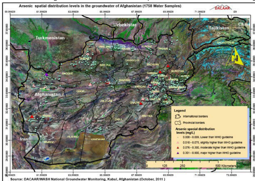
Figure 69 Arsenic distribution
