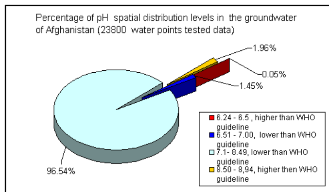
Figure 45 Percentage of ph distribution in the groundwater
