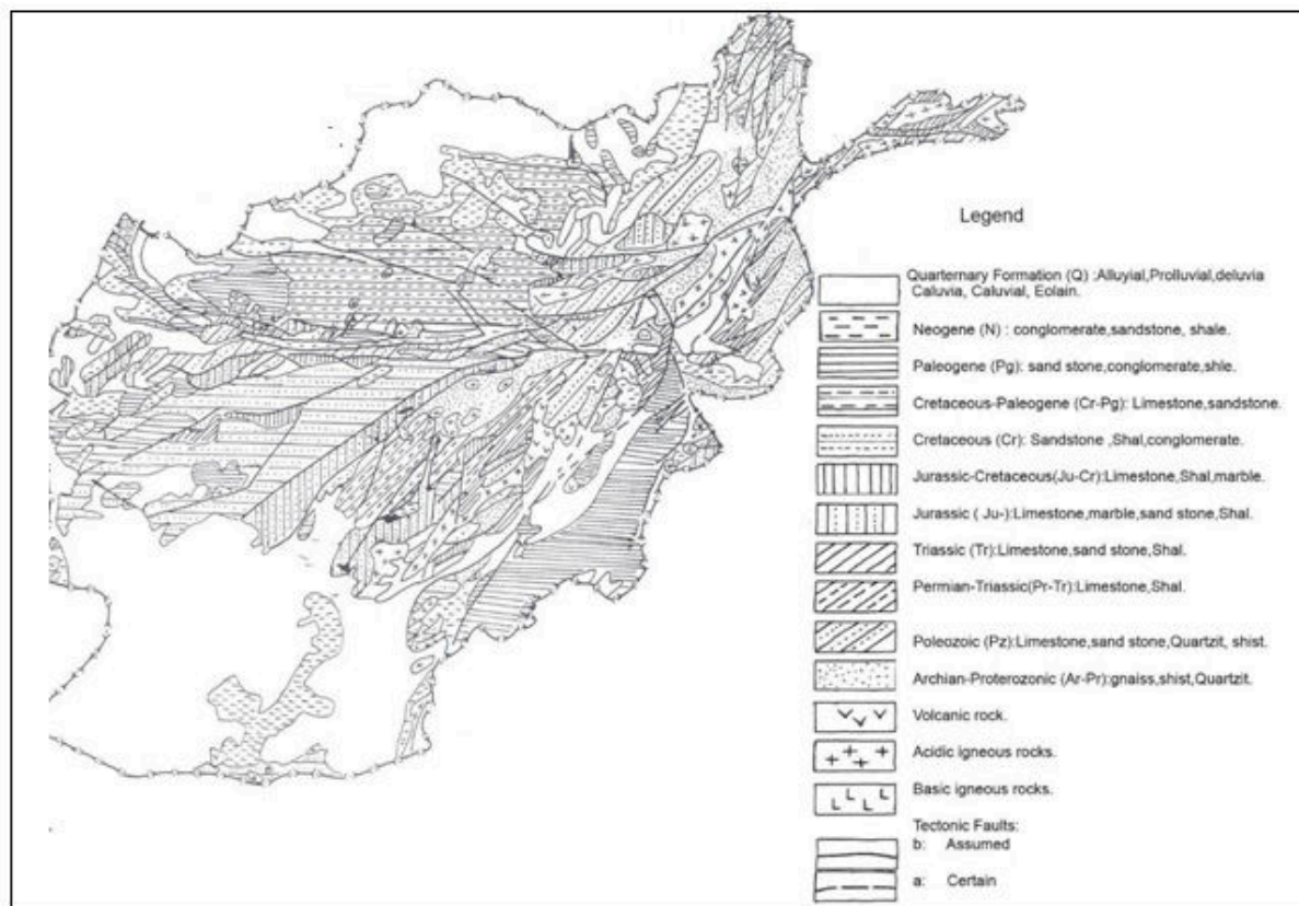
Geological Map of Afghanistan (W.A. Slawin, 1984)
