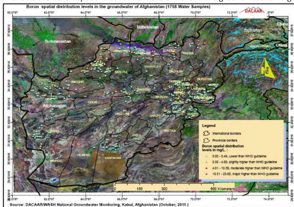
Figure 67 Boron distribution in groundwater
